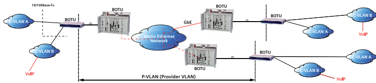
100 Mbit/s Connections via Metro Ethernet Network
