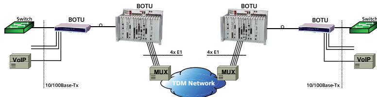
8 Mbit/s Ethernet Leased Lines over SDH/TDM Networks
